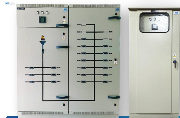
DB : DISTRIBUTION BOARD
